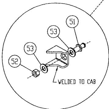
STRIKER BOLT DETAIL 4X SCALE
