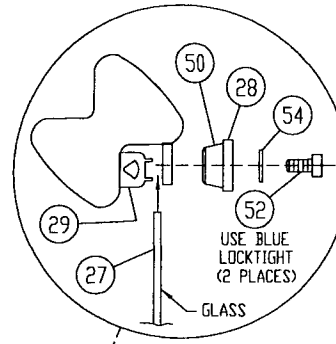
WINDOW CLAMP INSTALL 5X SCALE
