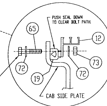
TYPICAL BOTTOM EDGE BOLTING PATTERN 5X SCALE
