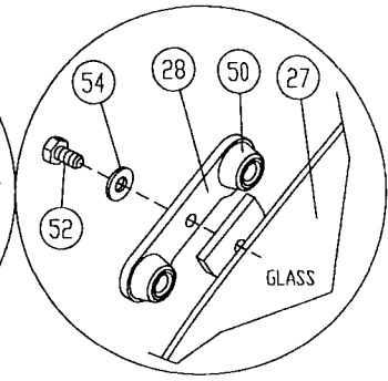
WINDOW CLAMP INSTALL ALTERNATE VIEW 5X SCALE
